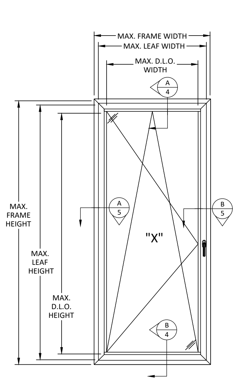
ELEVATIONS
