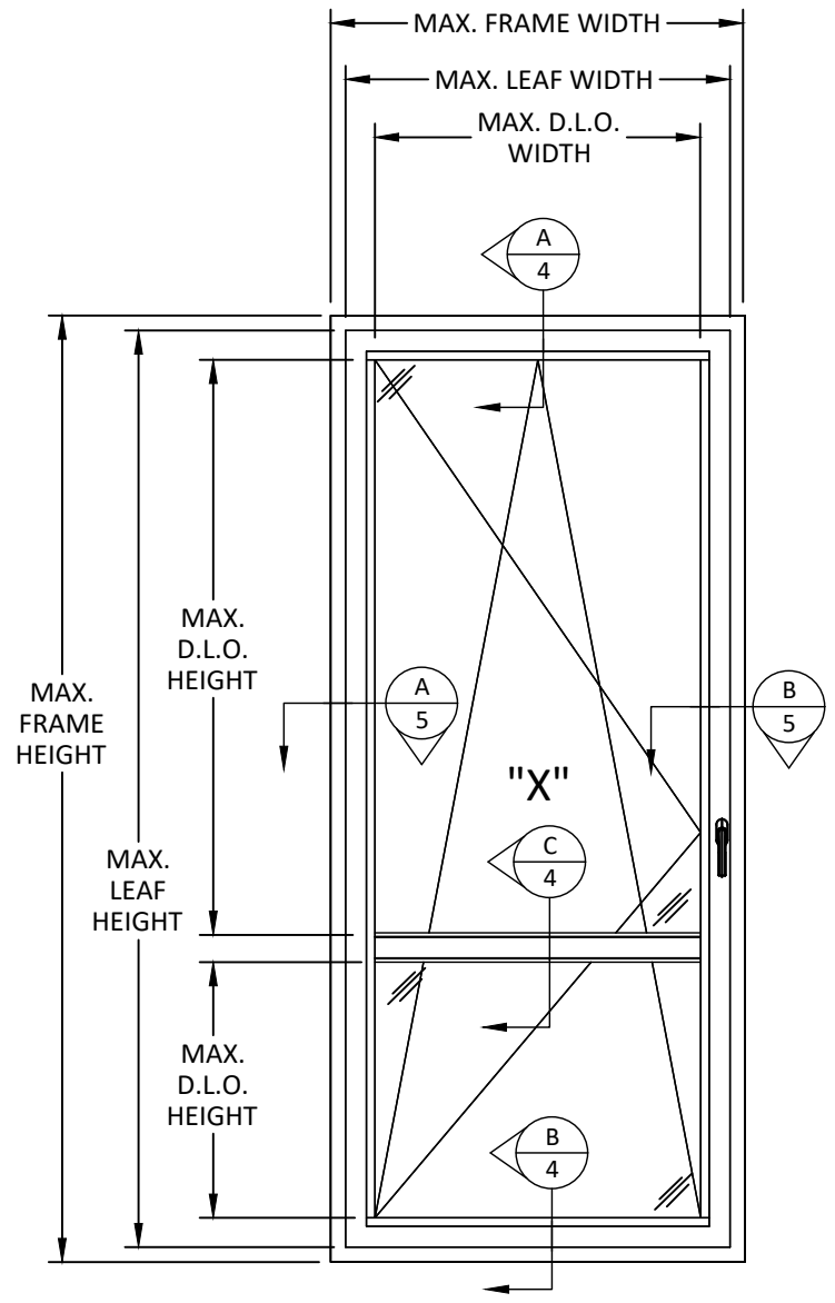
ELEVATIONS
